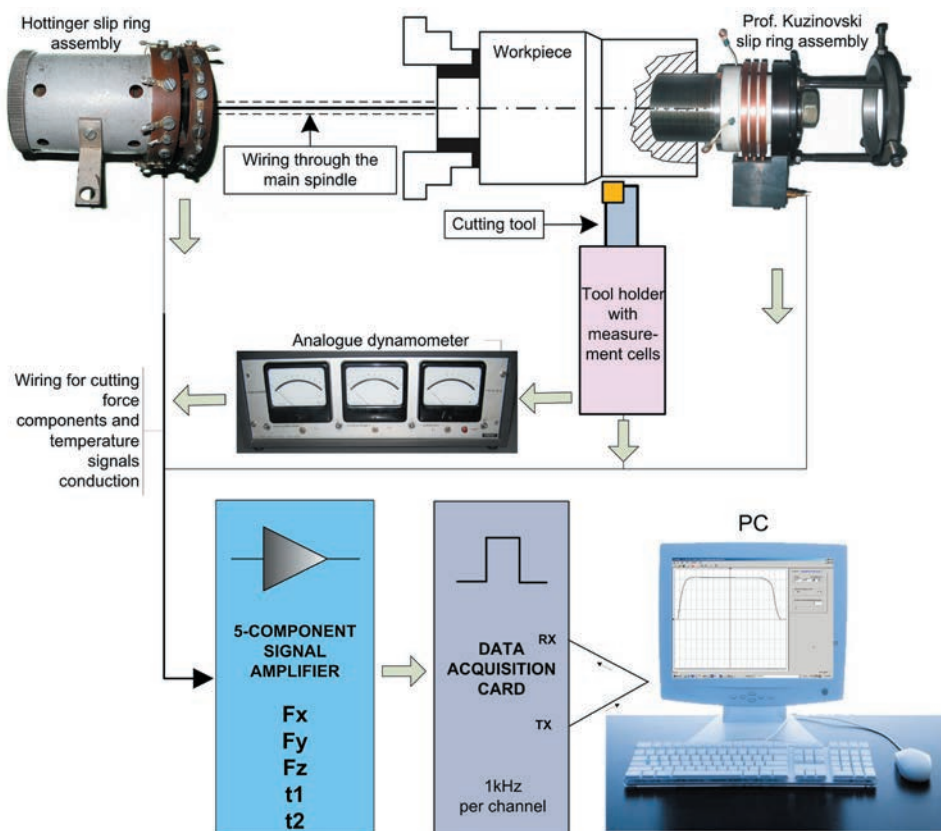
Fig. 1. Computer aided system for investigation of cutting forces and temperature in turning [5]
