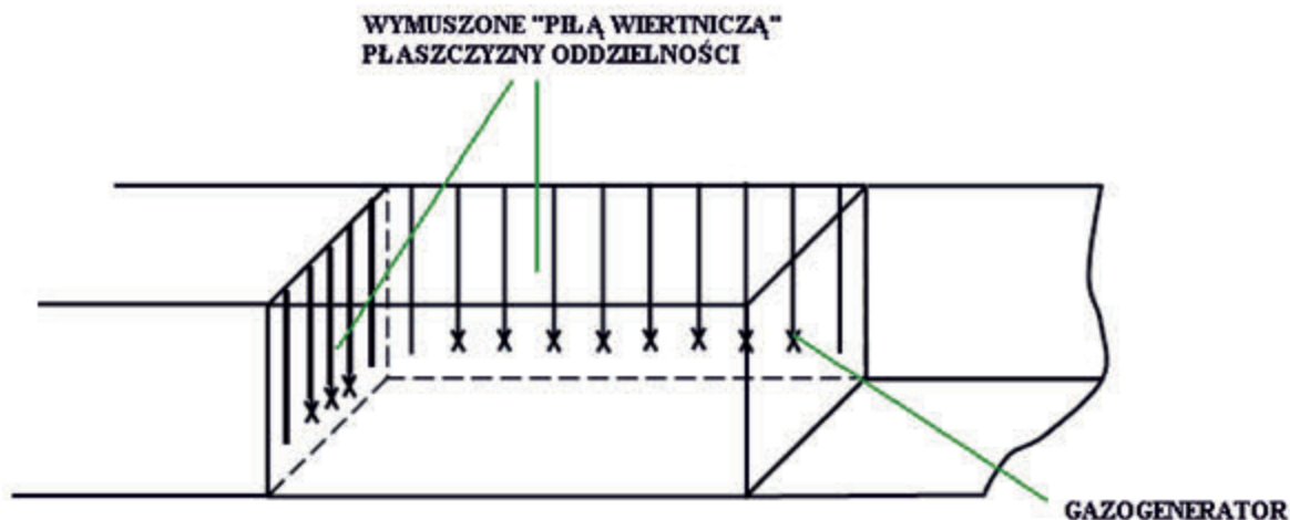
Rys. 2. Zasada odpajania bloków gazogeneratorem Fig. 2. The rule of gasgenerator operation
